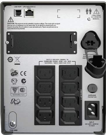
[SMT1000I]
